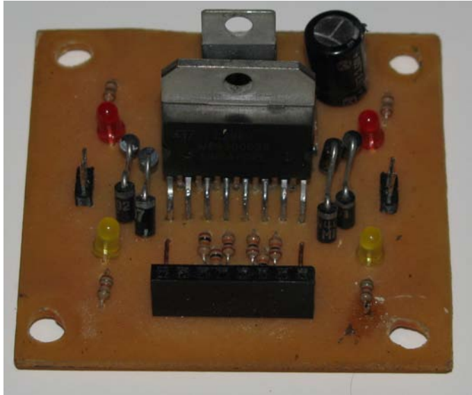
Figure 3-16. Here is the popular L298N dual 2amp H-bridge motor-controller on a homemade PCB. The other components include a 7805 5v regulator, a few EMF protection diodes, a capacitor, and some direction LEDs. This board can be used to control the speed and direction of two independent DC motors.
