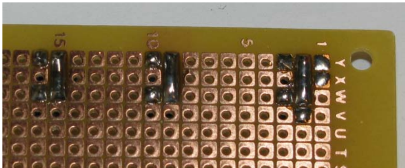
Figure 4-10. Make a “solder-bridge” between the anode of the emitter and the collector of the photo-transistor
